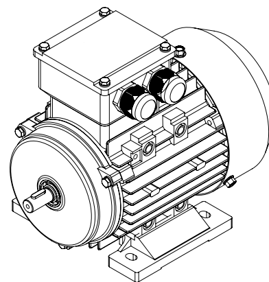
1ALZ-63-B3 Mounting diagram
